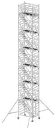
RS4S135x185x1200C
