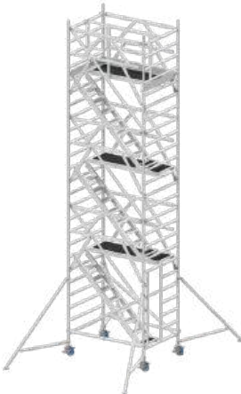
RS4S135x185x600C
