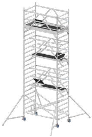
RS4S135x245x600
