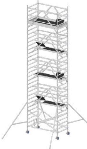
RS4S135x245x800
