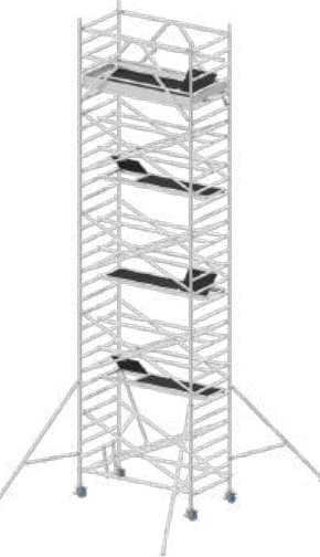
RS135x245x800
