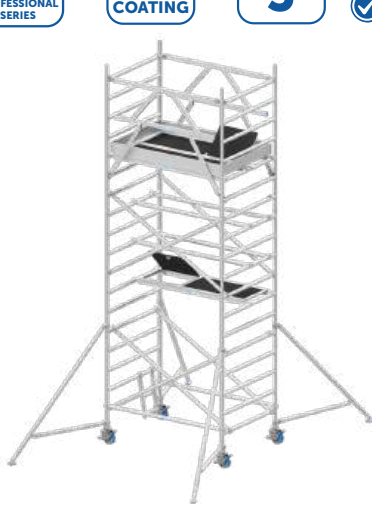
RS135x185x400
